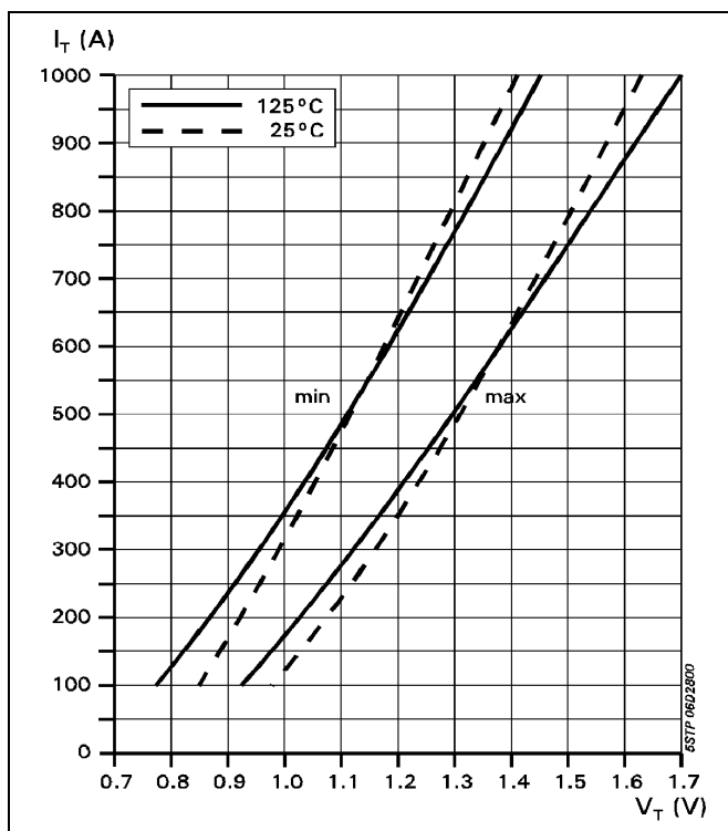
Fig. 2 On-state characteristics.
