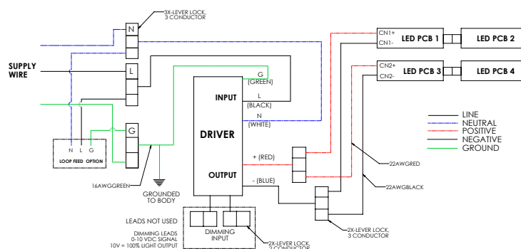
4 Foot UNV1 Wiring Diagram - Figura 10B
