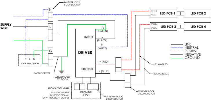
4 Foot UNV1 Wiring Diagram - Figure 10B
