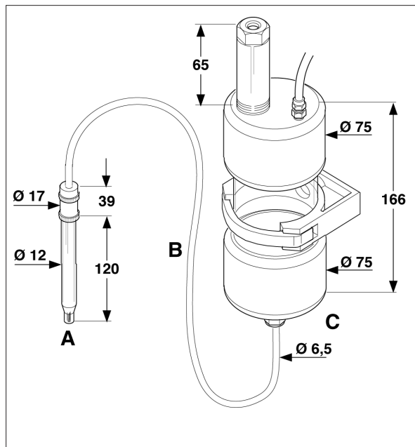
Figure 1: SB20 drawing
