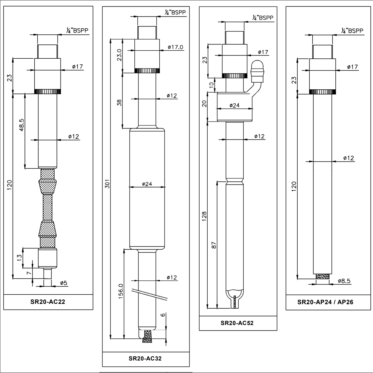
Figure 2: SR20 dimensions
