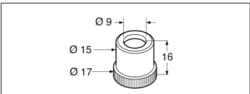
Figure 4: K1500DW (set of 12 cable nuts)
